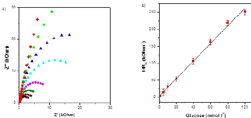
Figure 1. a) Impedance response of GOD/opPy/Au \mu Ts/Pt electrode in solutions of glucose in phosphate buffer at pH 7, for concentrations ranging from 1.0 mM, to 100.0 mM, b) Calibration curve 1/R_s vs. glucose concentrations
