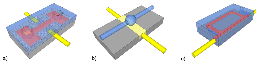
Figure 1 – Schematic representation of a) photonic crystal resonator, b) bubble resonator, c) ring resonator.
